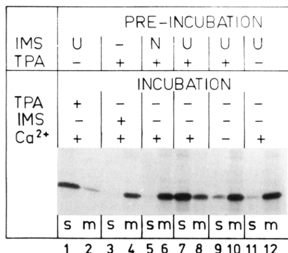
FIGURE 5: Interaction of the releasing factor with TPA. Photoaffinity labeled mitochondria were separated into mitoplast and intermembrane space fractions. Preincubation: One out of five aliquots of intermembrane space proteins (+IMS) (125 \mu g each) was treated with 1 mM NEM (N) (15 min, 0 ^{\circ} C, terminated with 2 mM DTT). The others remained untreated (U). All samples and a control, lacking intermembrane space proteins (-IMS), were incubated with TPA (5 min, 4 ^{\circ} C) and then passed through a 2-mL column of Sephadex G-10. The eluate (500 \mu L) was concentrated 5-fold by ultrafiltration through an Amicon XM-300 membrane. Incubation: Six aliquots of purified mitoplasts (400 \mu g each) were supplemented with 80 \mu g of pretreated or untreated intermembrane space proteins (IMS) or with the control sample (-IMS) and incubated with or without \text{Ca}^{2+} plus TPA. All samples were separated into mitoplasts (m) and soluble proteins (s) by two-step sucrose gradient centrifugation and analyzed by SDS-PAGE (12%) and fluorography.
