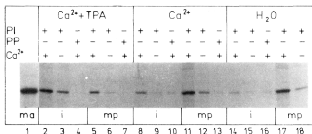
FIGURE 3: Ca 2+ -dependent phosphorylation of the cAMP receptor. Mitochondria (1.2 mg) were incubated with H 2 O, Ca 2+ , or Ca 2+ plus TPA and separated into mitoplast (mp) and intermembrane space fraction (i). Both fractions, recovered by centrifugation or precipitation, respectively, and solubilized in column buffer plus 0.5% MEGA 10, were subjected to cAMP-Sepharose affinity chromatography. Three aliquots of the protein of each fraction, eluted by 0.1 M cAMP, received, after dialysis, PEG precipitation, and solubilization in kinase buffer, either 100 \mu M Ca 2+ plus phosphatase inhibitors (PI), 100 \mu M Ca 2+ plus 2 mg/mL protein phosphatase 2A (PP), or 50 \mu M EGTA plus phosphatase inhibitors (PI) (see legend to Figure 1). All samples were incubated with 250 nCi of [ \gamma - 32 P]ATP (30 min, 30 °C). The reaction was terminated by precipitation with 5% TCA, and the pellets, after being washed, were analyzed by SDS-PAGE (12%) and autoradiography. Total protein from Ca 2+ /TPA-treated and photoaffinity labeled mitochondria was run on the same gel as a marker (ma).
