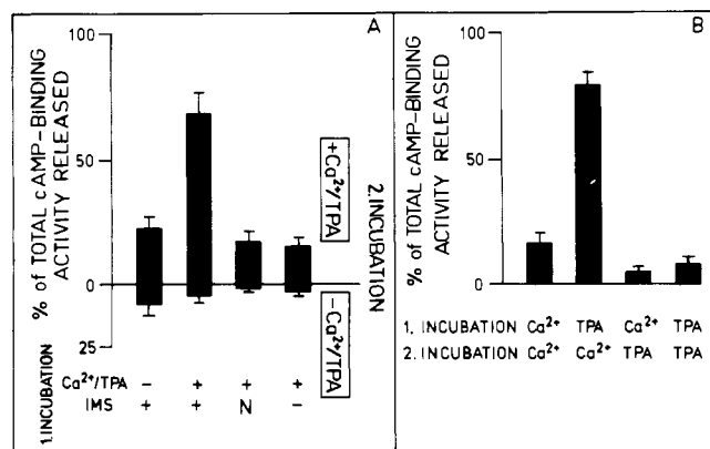
FIGURE 7: Association of the releasing factor with mitochondrial membranes. Panel A: Mitoplasts, deprived of cAMP-binding activity (400 \mu g each), were supplemented with untreated (+IMS) or NEM-treated (N) (1 mM, 15 min, 0 °C, stopped with 2 mM DTT) intermembrane space proteins or were not supplemented (-IMS) and were incubated with or without Ca 2+ plus TPA (1. INCUBATION). The mitoplasts, recovered from two-step sucrose gradients, were assayed for association of the releasing factor in the presence or absence of Ca 2+ plus TPA (2. INCUBATION). Panel B: The experiment followed that in panel A except that both incubations were carried out in the presence of untreated intermembrane space proteins and either Ca 2+ or TPA.
