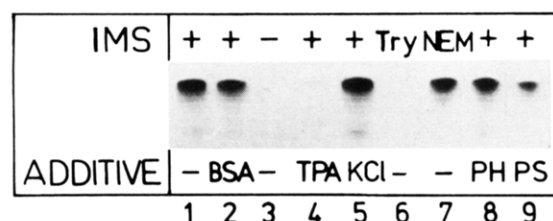
FIGURE 6: Identification of a phorbol ester binding protein in the intermembrane space. A total of 200 \mu g of intermembrane space proteins (2 mg/mL in assay buffer), either untreated (+IMS) or pretreated with trypsin (Try) or NEM, was supplemented with 40 nM [ ^3\text{H} ]PDB (200 nCi), 200 \mu M PMSF, 1 \mu M leupeptin, 1 \mu M pepstatin, 10 \mu g/mL \alpha_2 -macroglobulin, and 100 \mu M EDTA, incubated in the presence of either 0.5% BSA, 3 \mu M TPA, 250 mM KCl, 3 \mu M phorbol acetate (PH), or 5 \mu M phosphatidylserine (PS) in a total volume of 200 \mu L (15 min, 4 ^{\circ} C), and then spun through a 1-mL column of Sephadex G-10. The eluate (250 \mu L) was concentrated 5-fold by centrifugation through an Amicon microconcentrator (XM-300 membrane) and electrophoresed (12% polyacrylamide gel) in the absence of SDS and mercaptoethanol and the presence of 200 \mu M PMSF overnight at 4 ^{\circ} C. Separated proteins were transferred to a nitrocellulose filter (Towbin et al., 1979) for 15 min at 4 ^{\circ} C (absence of SDS and urea, presence of 200 \mu M PMSF). The dried filter was autoradiographed.
