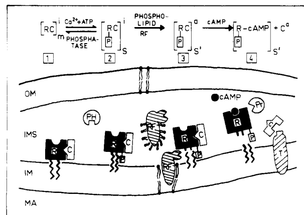
FIGURE 8: Working model for release of the mitochondrial cAMP receptor. (1) The cAMP-dependent protein kinase, consisting of a cAMP-binding regulatory subunit (R) and a catalytic subunit (C), is associated with the inner membrane (IM) of yeast mitochondria via the phosphatidylinositol membrane anchor of the R subunit. This membrane-bound (m) complex, [RC], is inactive (i) because it fails to dissociate into the subunits despite its ability to bind cAMP. (2) The interaction of the R subunit with the inner membrane is weakened by its \text{Ca}^{2+} -dependent phosphorylation, causing partial release (S) of the still inactive complex [RC] and an increased accessibility of the lipid anchor for lipolytic attack. This process is reversed by a soluble phosphatase (PH). (3) The soluble releasing factor (RF) of the intermembrane space binds to phospholipids, presumably at the inner face of the outer membrane (OM). The lipids are then transferred to the outer face of the inner membrane, whereby the releasing factor itself associates with the inner membrane. The intrinsic phospholipase activity of this NEM-sensitive protein then cleaves the lipid anchor of the R subunit, causing irreversible release (S') of the complex [RC] into the intermembrane space. (4) The soluble complex [RC] can be activated (a) since binding of cAMP now causes its dissociation. The R subunit is then readily digested by proteases (Pr), and the active C subunit phosphorylates a 40-kDa target protein (T) of the inner membrane, thereby causing signal transmission into the matrix (MA).
