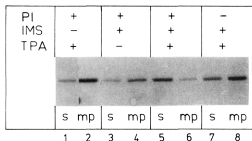
FIGURE 1: Two-step release of the cAMP-binding protein. Photoaffinity labeled mitochondria (1.6 mg) were incubated with \text{Ca}^{2+} , supplemented with phosphatase inhibitors (final concentrations: NaF, 1 mM; G-3-P, 2 mM; sodium molybdate, 5 mM; \text{NaPP}_i , 10 mM) and EGTA (final concentration 100 \mu\text{M} ), and converted to mitoplasts. After centrifugation through a 2-mL cushion of 0.1 M sucrose, four aliquots of the resuspended mitoplasts (4 mg/mL in assay buffer plus 0.5 mM EGTA) were incubated in the presence or absence of 80 \mu\text{g} of intermembrane space proteins with or without TPA and phosphatase inhibitors (PI) (see above). The mixtures were separated into mitoplasts (mp) and soluble proteins (s) by two-step sucrose gradient centrifugation and precipitated with 66% (\text{NH}_4)_2\text{SO}_4 . The TCA- and acetone-washed pellets were analyzed by SDS-PAGE (12%) and fluorography.
