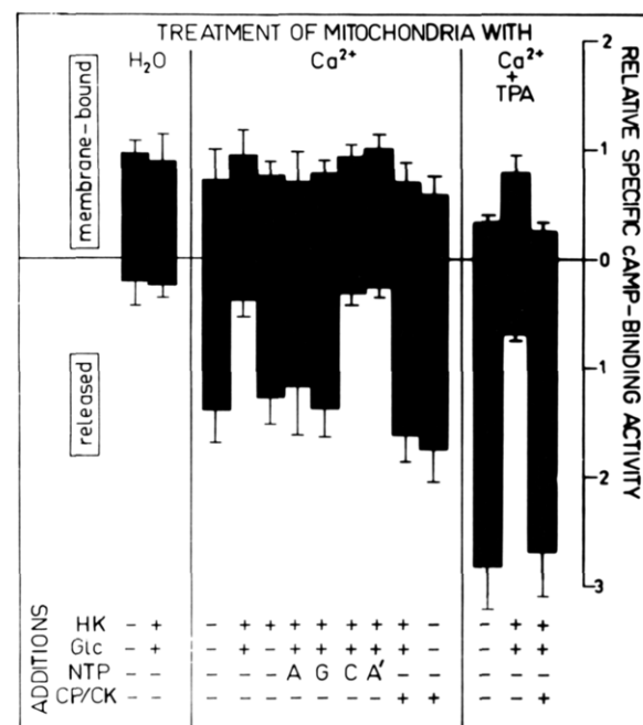
FIGURE 2: Energy requirement of the releasing process. Mitochondria (2 mg/mL in SEM buffer) were incubated in the presence or absence of 25 units/mg hexokinase (HK) with or without 10 mM glucose (Glc) (10 min, 30 °C) and subsequently supplemented with either 2 mM (final concentration) ATP (A), 2 mM GTP (G), 5 mM CTP (C), 10 mM AMPPCP (A'), or 20 mM creatine phosphate, 5 \mu\text{g} /mL creatine kinase, and 2 mM ADP (CP/CK). After further incubation (5 min, 30 °C) the samples were cooled on ice and aliquots treated with or without \text{Ca}^{2+} and TPA and centrifuged through a 0.5-mL cushion of 0.4 M sucrose. The resuspended mitochondria (2 mg/mL in assay buffer) were separated into mitoplasts (membrane bound) and intermembrane space proteins (released). Both fractions were assayed for cAMP-binding activity. The relative specific cAMP-binding activity of untreated solubilized mitochondria was set as 1 (0.37 pmol/mg of protein).
