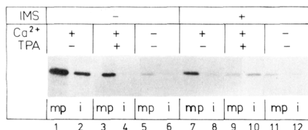
FIGURE 4: Phosphorylation of the cAMP receptor during its release. Two aliquots of mitoplasts (1.2 mg each) (2.5 mg/mL in kinase buffer plus 50 mM sucrose, 2 \mu Ci of [ \gamma - 32 P]ATP, and phosphatase inhibitors, see legend to Figure 1) were supplemented with 480 \mu g of intermembrane space proteins (+IMS) or not supplemented (-IMS). Both samples were divided into three aliquots and incubated with either Ca 2+ alone or Ca 2+ plus TPA or 50 \mu M EGTA (30 min, 30 °C). Mitoplasts (mp) and intermembrane space proteins (i), recovered from a two-step sucrose gradient, were supplemented with column buffer plus 0.5% MEGA 10, applied to a cAMP-Sepharose column (1 mL), eluted, and analyzed by SDS-PAGE (12%) and autoradiography.
